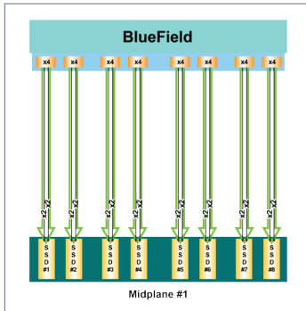
Figure 1. 8 SSD Configuration (2U platform)
