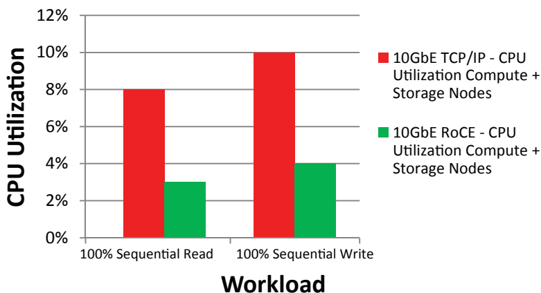
Total CPU Utilization @ 512KB Block Size [%] Lower is Better
