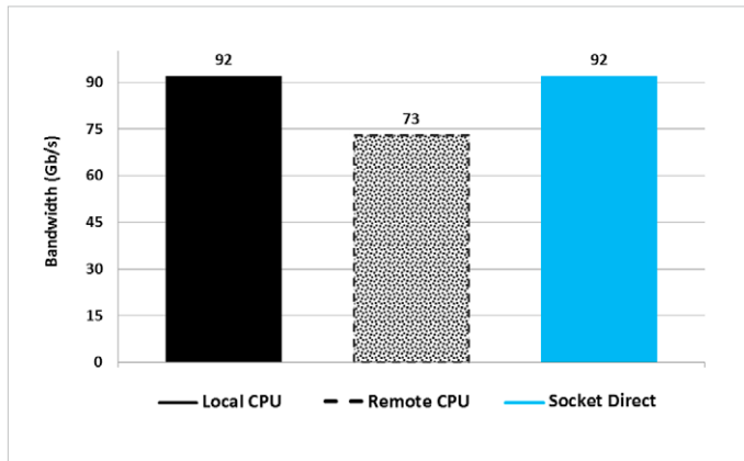
Figure 9. RoCE RDMA Throughput
