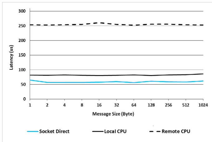
Figure 5. Average Latency
