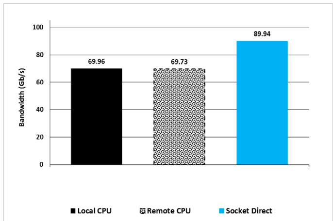
Figure 7. Load on the Inter-processor Bus
