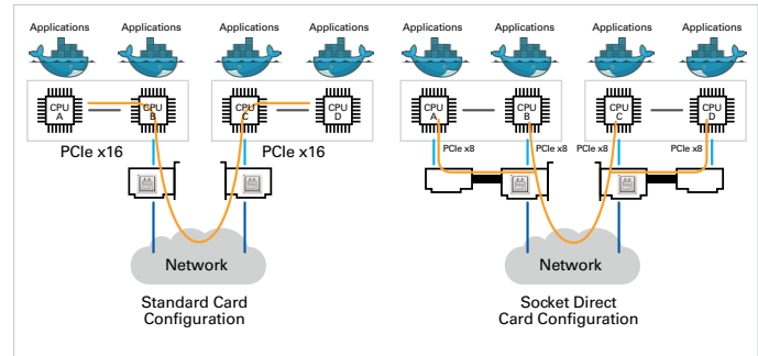
Figure 4. Standard Card Configuration versus Socket Direct Card Configuration (tests setup)
