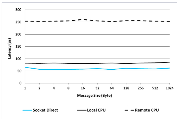
Figure 5. Average Latency
