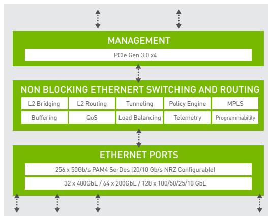
High Level System Block Overview
