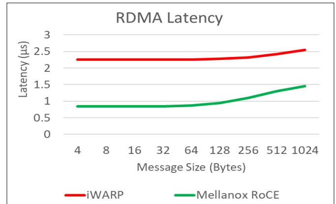
4 Node Microsoft S2D Cluster over Lossy Network
