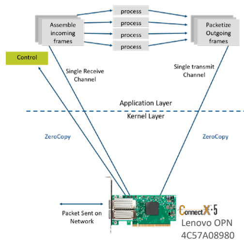
Figure 3: Smart Protocol Offload Enables Kernel Bypass
