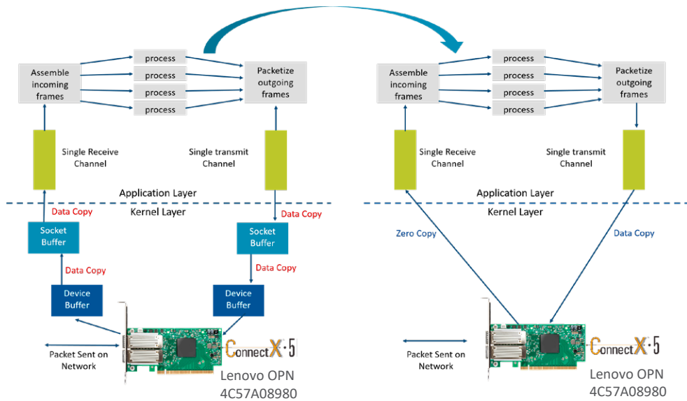
Figure 1: Zero-Copy with Mellanox Rivermax and Lenovo Adapters
