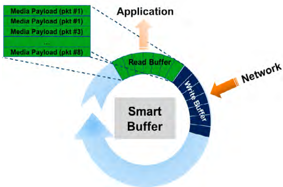
Figure 2: Smart Buffer Management with Mellanox Rivermax
